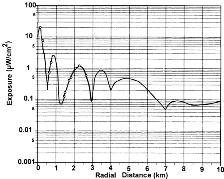
Figure 30: The measured and estimated power density (exposure in \mu\text{W}/\text{cm}^2 ) with distance from the Sutra Tower. Circles show measurements. The line follows measurement points and the radial pattern of a typical UHF transmission beyond 3 km. From Hammett and Edison (1997) and readings taken by the author in 1999.
