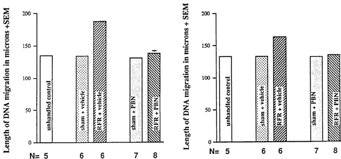
Figure 24: Effect of treatment with PBN for RFR-induced increase in DNA single-strand (left) and double-strand (right) breaks in rats brain cells. Data was analysed using the one-way ANOVA, which showed a significant treatment effect ( p < 0.001 ) for both cases. "vehicle" involves injecting with the physiological saline without the active substance. Lai and Singh (1997).
