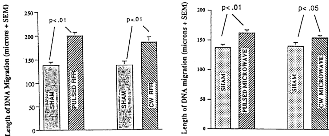
Figure 22: Single-strand (left) and double-strand (right) breaks in brain cells of rat after exposure to pulsed or continuous-wave RFR. Each bar represents data from 8 rats, Lai and Singh (1996).
