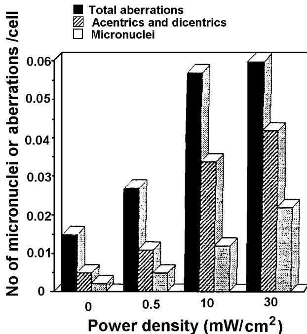
Figure 12: The relation of total chromosome aberrations, micronuclei and specific chromosome aberrations for each cell in human lymphocyte cultures in the dose of microwave radiation in vitro, Garaj-Vrhovac et al. (1992)
