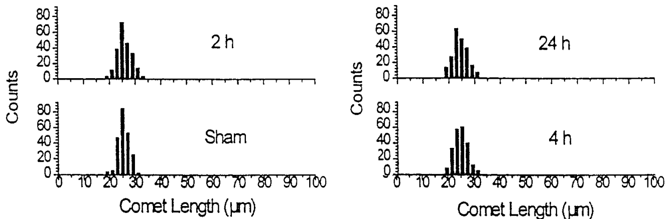
Figure 20: Frequency Distribution of Comet tail lengths for 2.45GHz exposed C3H10T1/2 cells, Malyapa et al. (1998).
