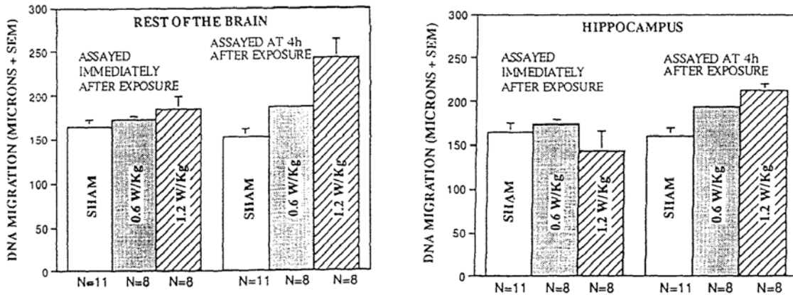
Figure 21: DNA single-strand breakage in cells from the rat brain and hippocampus, immediately after a 2 hr exposure to a whole body SAR of 0.6 and 1.2 W/kg to 2.45 GHz microwave radiation, pulsed at 500 pps. N is the number of rats studied. Lai and Singh (1995).
