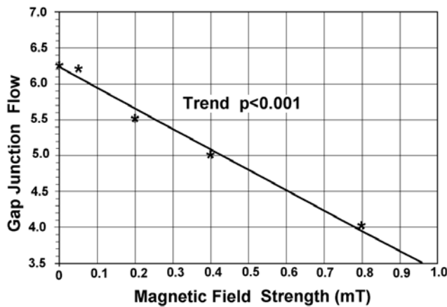
Figure 9: Gap junction flow as a function of 50 Hz magnetic field strength, Li et al. (1999).
